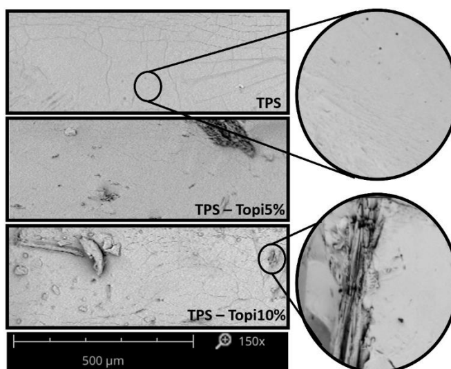
Figure 7. SEM micrographs of the cryofractured surface of cassava starch films without filler, 5% filler content and 10% filler content. Magnification used: 150×.
